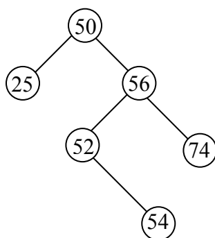
Fig W-1 Tree
