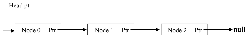
Fig. 49-2 Linked list using only forward pointing pointers (singly linked).
