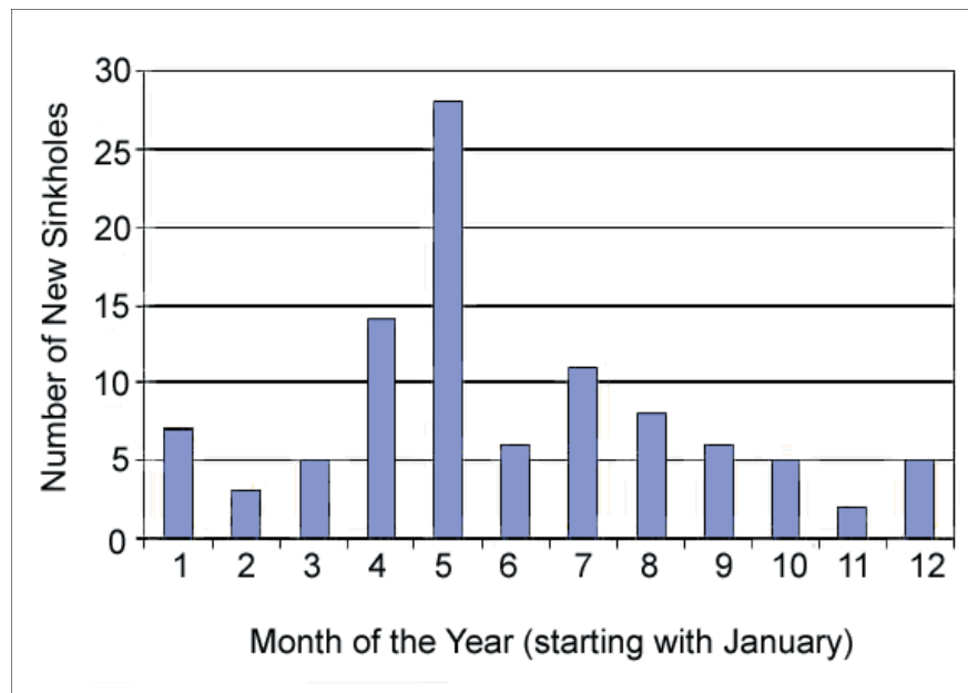
Figure 2: Number of new sinkholes in Orange and Seminole Counties, Florida by month of the year for the years 1961 through 1986. Note that the month of the year is represented with a number, starting with January as 1 and ending with December as 12.
